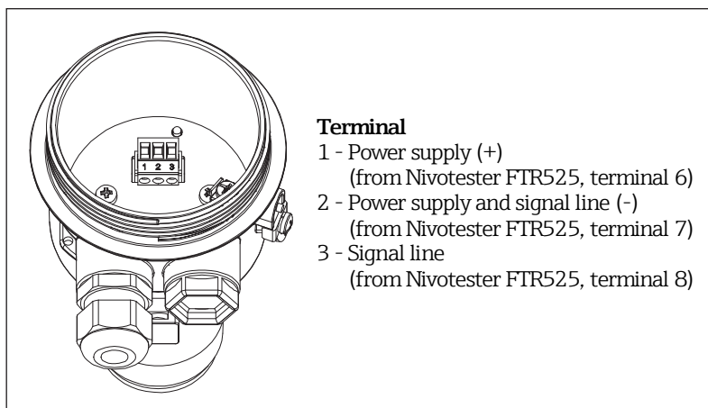
4 Terminal
