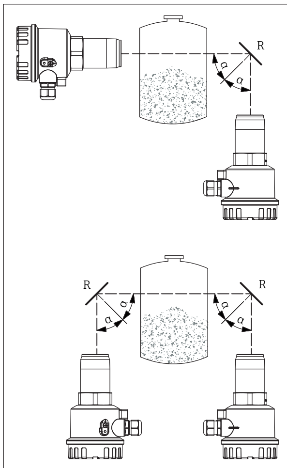
10 Reflector operation
